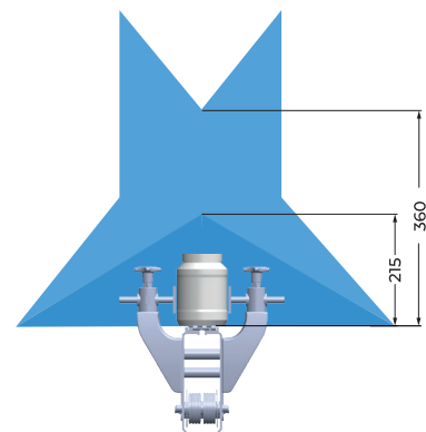
Beam geometry
