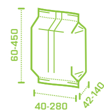
Gusseted bag
